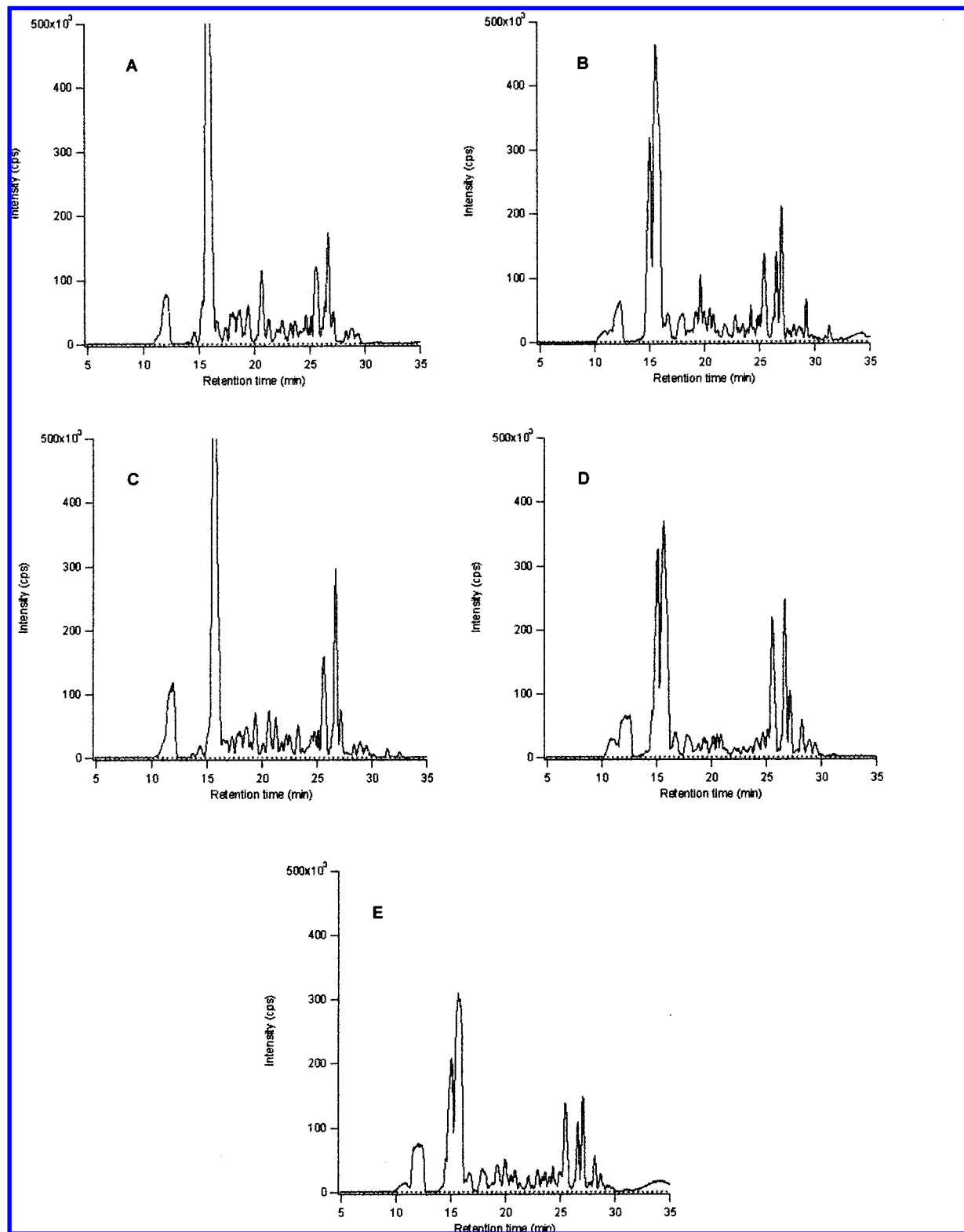
Figure 3. Base peak chromatograms of human milk oligosaccharides obtained from five different individual donors on day 6: donor 1 (A); donor 2 (B); donor 3 (C); donor 4 (D); donor 5 (E).
